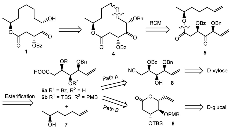
Scheme 1. Retrosynthetic Analysis of Sporiolide A (1)
