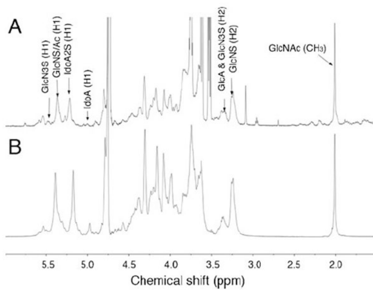
Fig. 4. 1 H NMR of bioengineered heparin (a) and commercial heparin sample (b)
