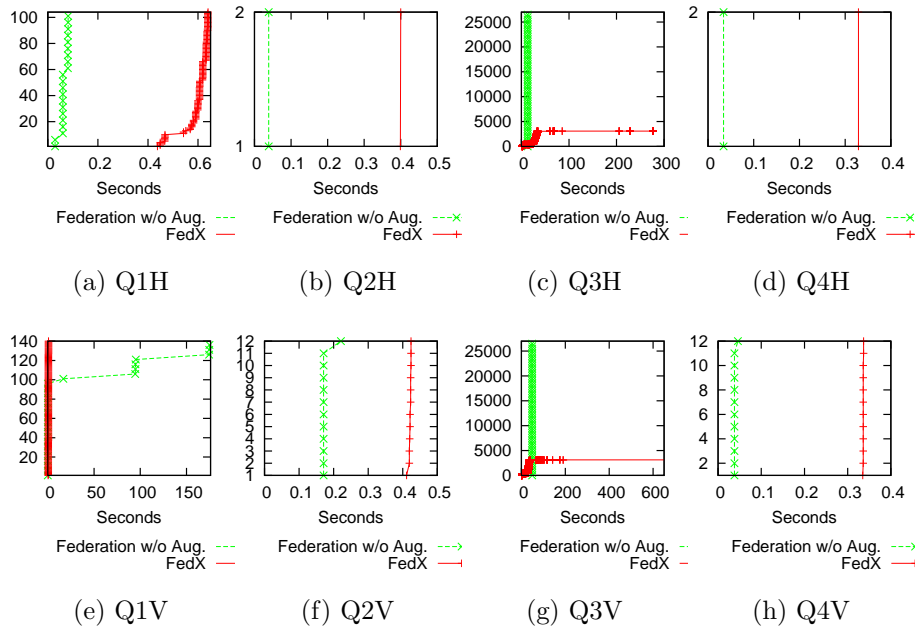
Figure 6.6: Queries Q1–Q4 results produced over time with no augmentation compared with FedX
