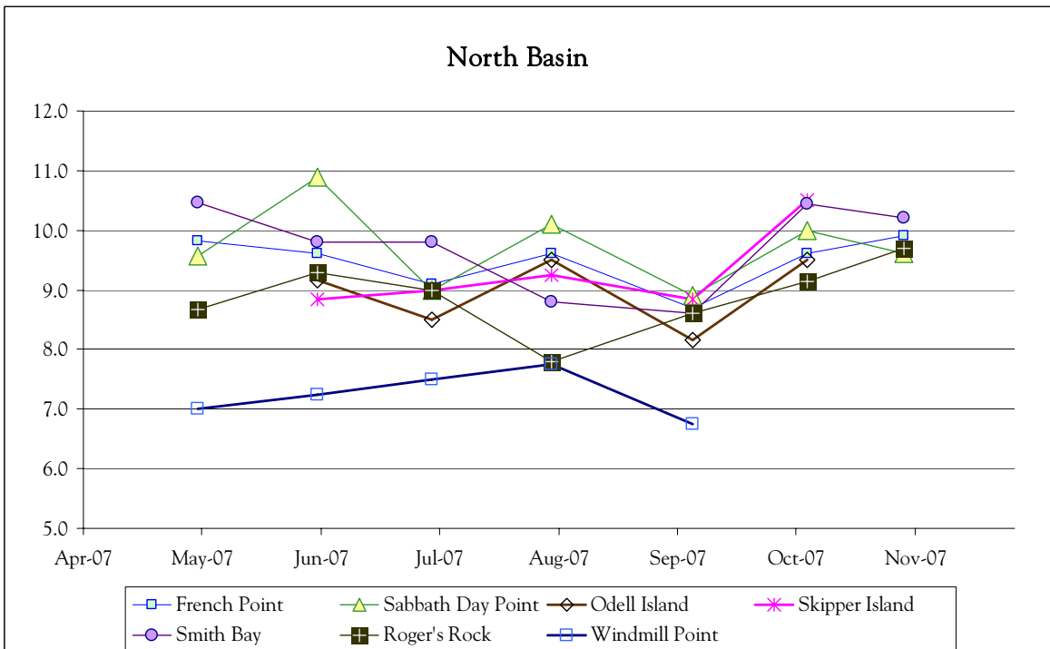
Figure 9. North Basin Secchi readings.
