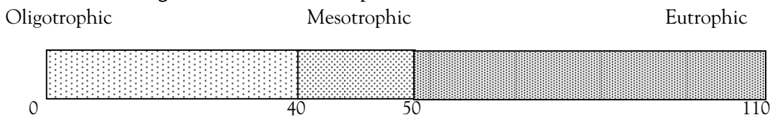
Figure 14. Carlson’s trophic state definition chart.
