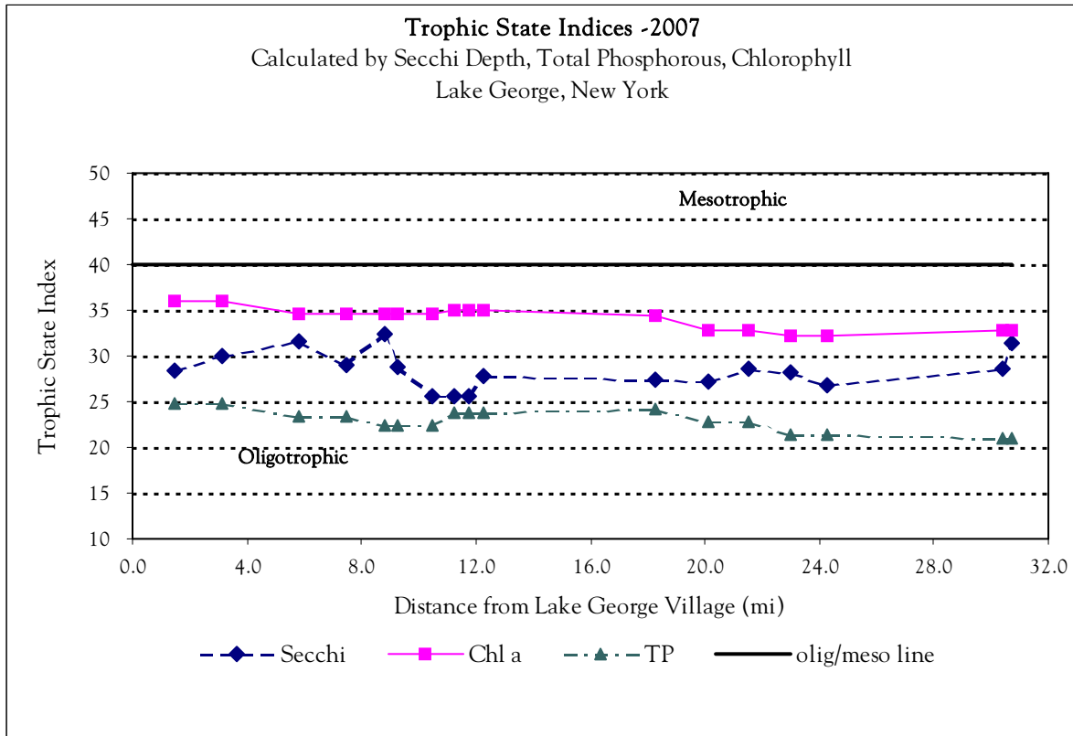
Figure 13. Trophic state indices for Lake George in 2007.
