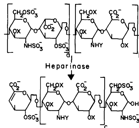
FIG. 1. Heparin is comprised of heparinase-cleavable (a) and uncleavable (b) glycosidic linkages. Depolymerization results in a disaccharide, tetrasaccharides, hexasaccharides, etc. when c = 0, 1, 2 etc. Structural variability includes the stereochemistry at the 5-position in the uronic acid residue and in substitution where X = \text{H} or \text{SO}_3^- and Y = \text{CH}_3\text{CO} or \text{SO}_3^- .
