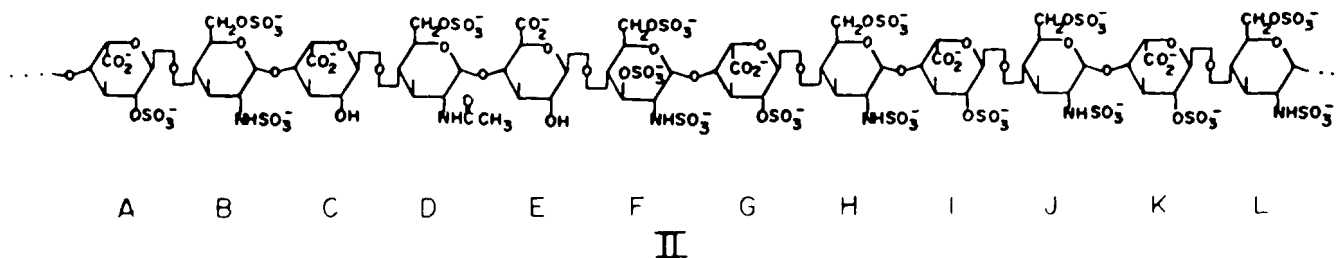
STRUCTURES I AND II
