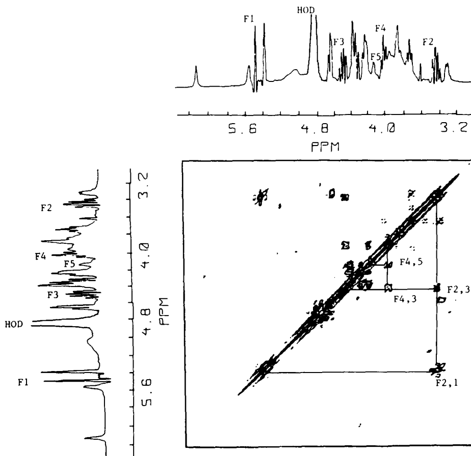
FIG. 4. Two-dimensional ^1\text{H} homonuclear COSY NMR of hexasaccharide I. The spectra was obtained on 12 mg of hexasaccharide I sodium salt in 200 \mu\text{l} of \text{D}_2\text{O} at pH 4.2. Assignments of specific peaks in the ^1\text{H} spectra are shown (see Table I for additional assignments). Off-diagonal peak connectivities used to demonstrate the presence of a 3-sulfated glucosamine residue at the reducing terminus of hexasaccharide I are shown.
