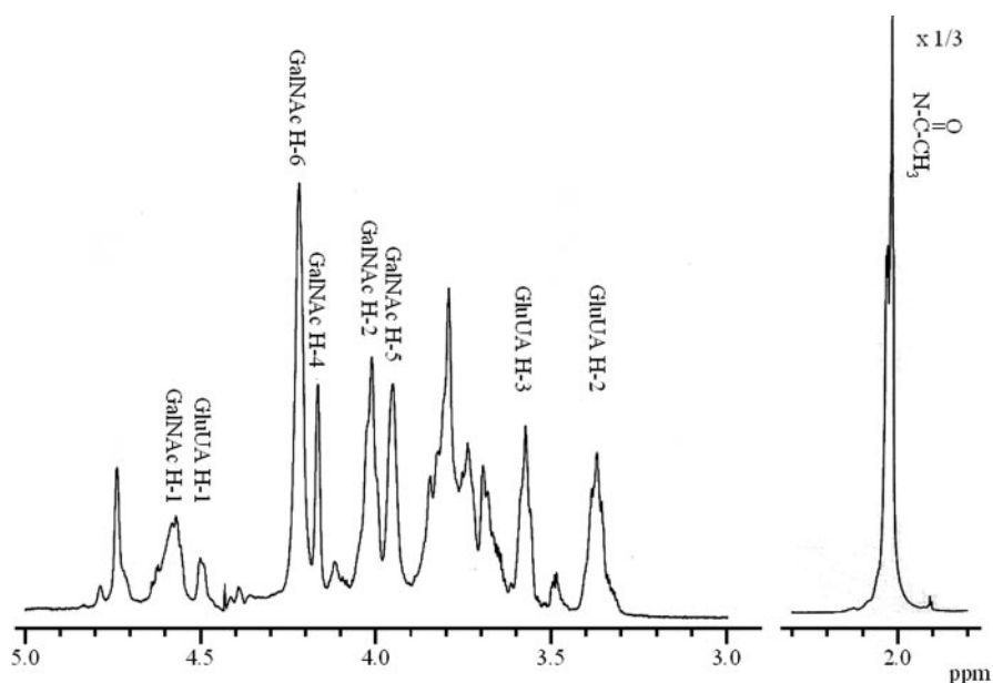
FIGURE 1. 1 H NMR spectrum of CS recorded in 2 H 2 O at 333 K. The peaks are labeled according to the main corresponding residues in the structure and the resonating proton. The height of the NHC(=O)CH 3 peak has been reduced to one-third to be in scale.
