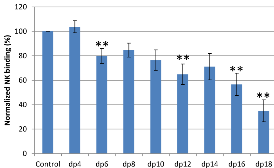
Figure 3. SPR competition study using heparin oligosaccharides. Top: Sensorgrams of solution heparin oligosaccharides/surface heparin competition. NK concentration was 2500 nM, and concentrations of heparin oligosaccharides in solution were 1000 nM). Bottom: Bar graphs (based on triplicate experiments with standard deviation) of normalized NK binding to surface heparin by competing with different size of heparin oligosaccharides in solution. Statistical differences were calculated using software SPSS version 14.0 at the 5% probability level (**, p < 0.05 ).
