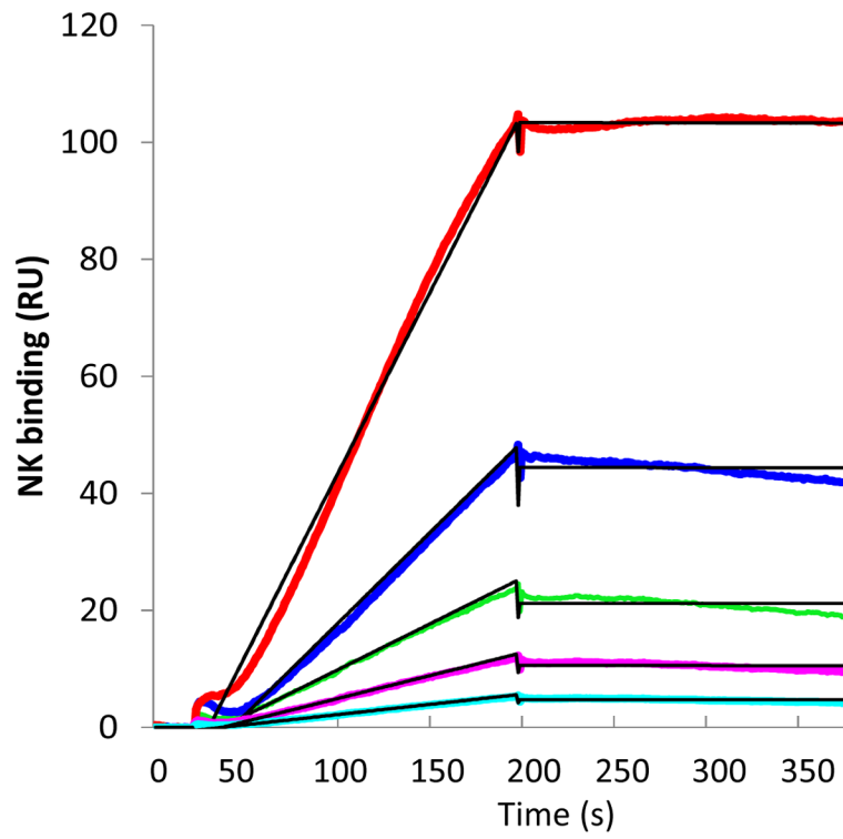
Figure 2. SPR sensorgrams of NK-heparin interaction. Concentrations of NK (from top to bottom): 2500, 1250, 630, 315, and 158 nM, respectively. The black curves are the fitting curves using models from BIAevaluate 4.0.1.
