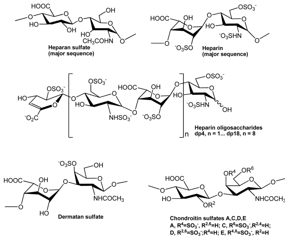
Figure 1. Chemical structures of heparin, heparin-derived oligosaccharides and other GAGs.
