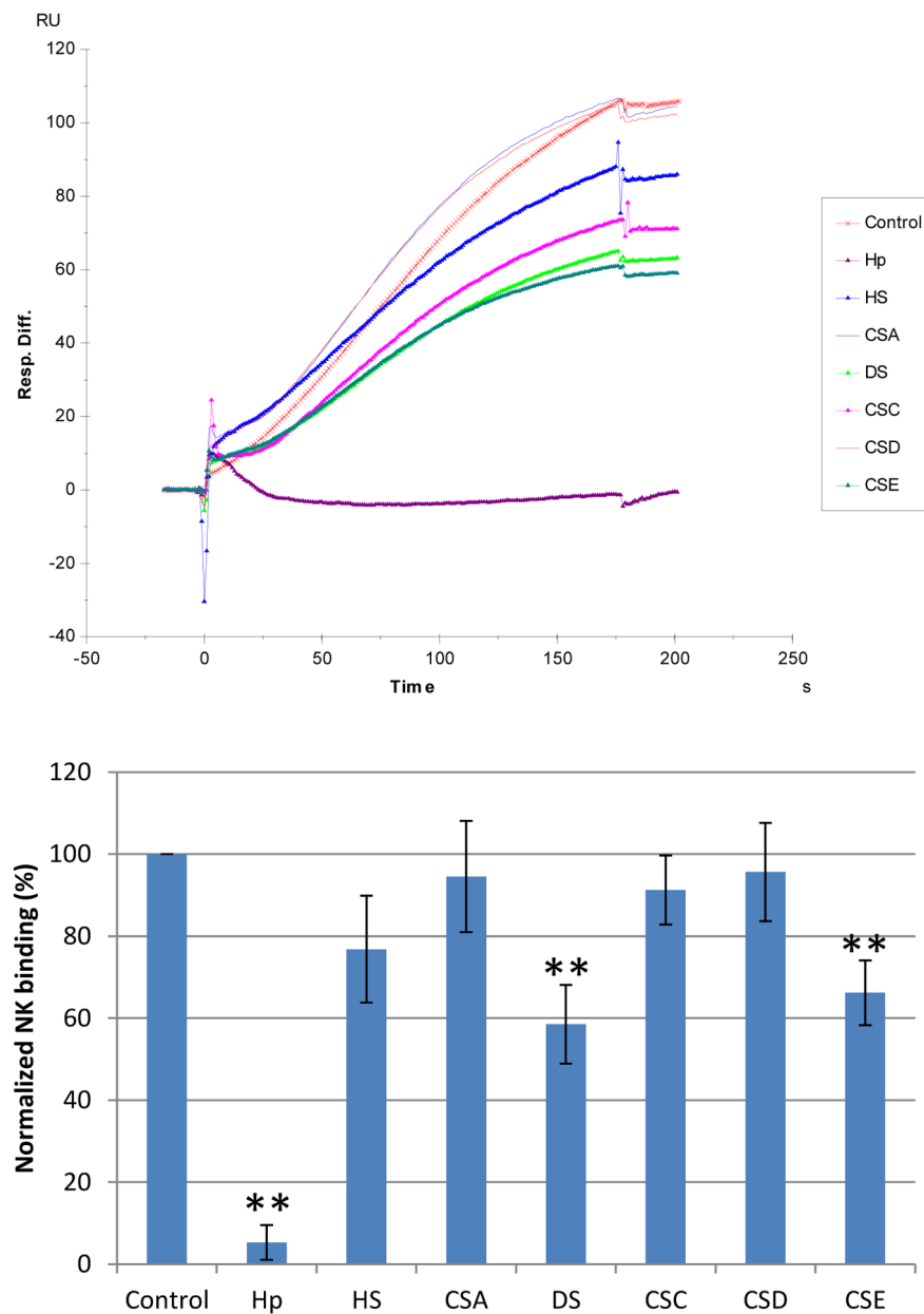
Figure 4. SPR competition study using different GAGs. Top: Sensorgrams of solution GAGs/surface heparin competition. NK concentration was 2500 nM, and concentrations of GAGs in solution were 1000 nM). Bottom: Bar graphs (based on triplicate experiments with standard deviation) of normalized NK binding to surface heparin by competing with different GAGs in solution. Statistical differences were calculated using software SPSS version 14.0 at the 5% probability level (**, p < 0.05 ).
