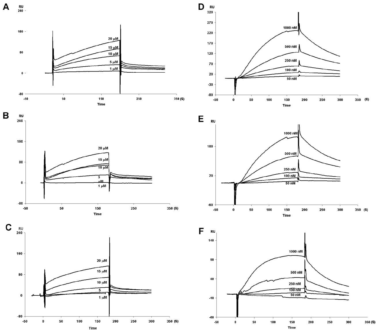
Figure 3. Sensorgrams showing the interaction of ATIII ( 20,15,10,5,1 \mu\text{M} ) with (A) LMWCPS1; (B) LMWCPS2; (C) LMWCPS3 and the interaction of HCII (1000, 500, 250, 100, 50 nM) with (D) LMWCPS1 ; (E) LMWCPS2; (F) LMWCPS3
