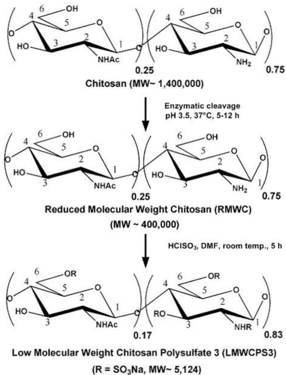
Scheme 1. Preparation of Low-Molecular-Weight Chitosan Polysulfate.
