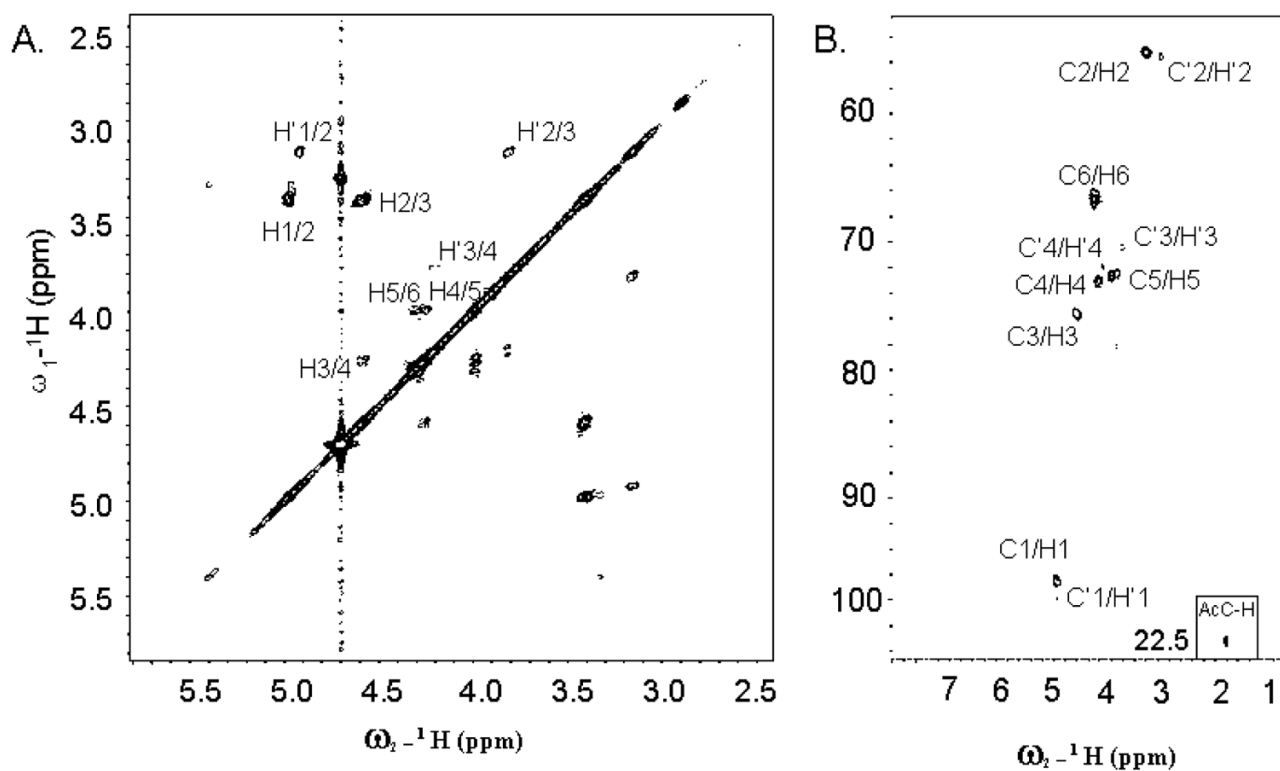
Figure 2. 2D NMR spectrum of LMWCPS1. A. ^1\text{H} - ^1\text{H} COSY of LMWCPS1. Two series of assignments, H is the residue of N -sulfoglucosamine (GS); H' is the residue of N -acetylglucosamine (GA); B. HMQC of LMWCPS1. Two series of assignments, C/H is residue of N -sulfoglucosamine (GS); C'/H' is residue of N -acetylglucosamine (GA).
