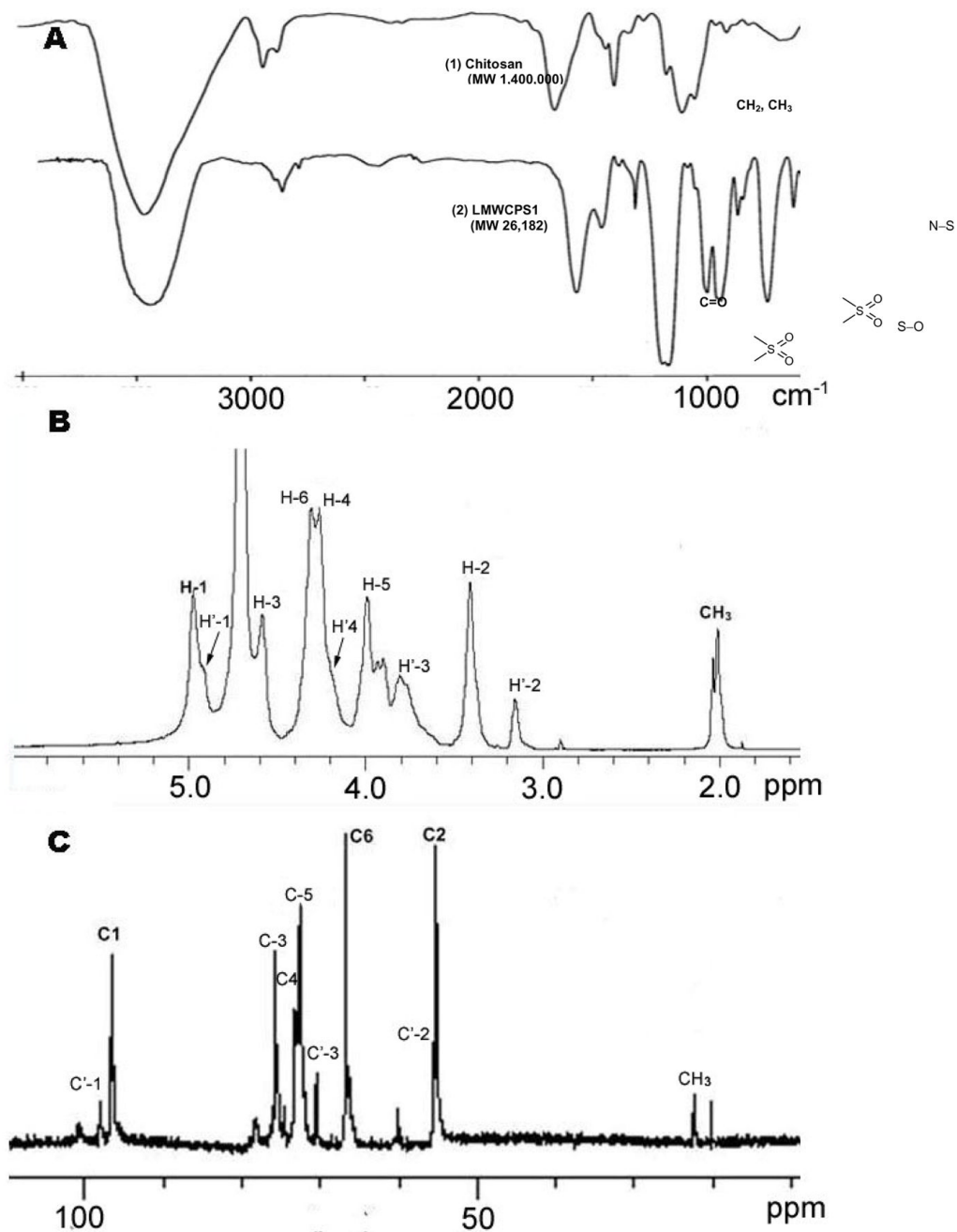
Figure 1. Characterization of LMWCPS1 A. IR spectra of (1) chitosan; (2) LMWCPS1 B. 1 H NMR spectrum. C. 13 C NMR spectrum.
