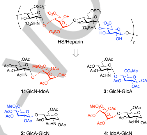
Figure 1. Representative structure found in HS/heparin and core disaccharide building blocks.
