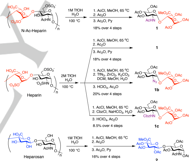
Scheme 1. Synthesis of GlcN-IdoA and GlcA-GlcN Building Blocks from Natural Polysaccharides. TfOH = trifluoromethanesulfonic acid, Ac = acetyl, TfN 3 = trifluoromethanesulfonyl azide, CbzCl = benzyl chloroformate.
