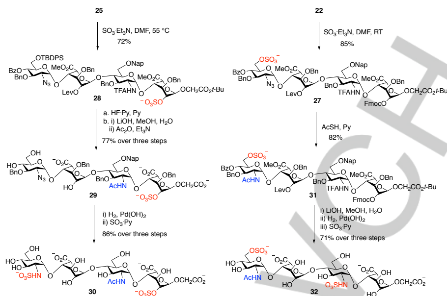
Scheme 5. Regioselective sulfation of the 2-O, 6-O and N positions to give tetrasaccharides bearing asymmetrical, regiodefined sulfation patterns.
